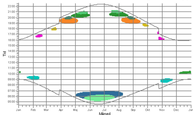
S5-B: Generisk 8MW-170 8000 170.0 !O! nav: 115,0 m (TOT:200,0 m) (22)
