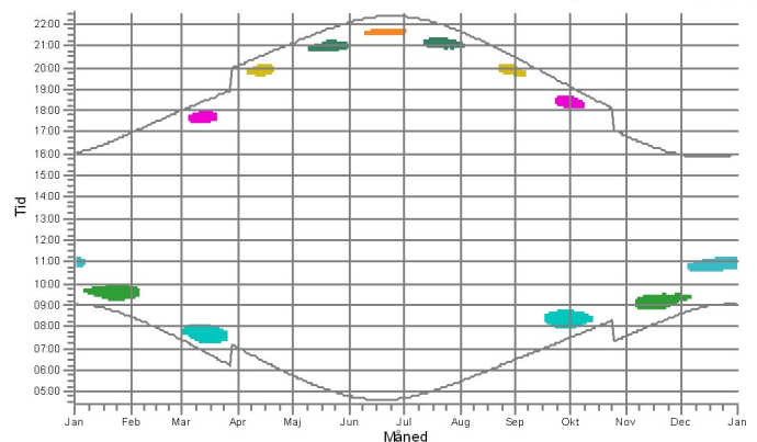
S3-B: Generisk 8MW-170 8000 170.0 !O! nav: 115,0 m (TOT:200,0 m) (25)
