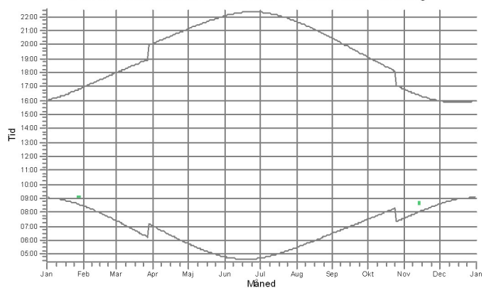
14: 57071500000037948: 600 kW NEG MICON - Bøvling
