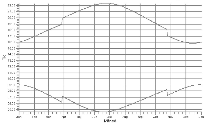
15: 57071500000037955: 600 kW NEG MICON - Bøvling
